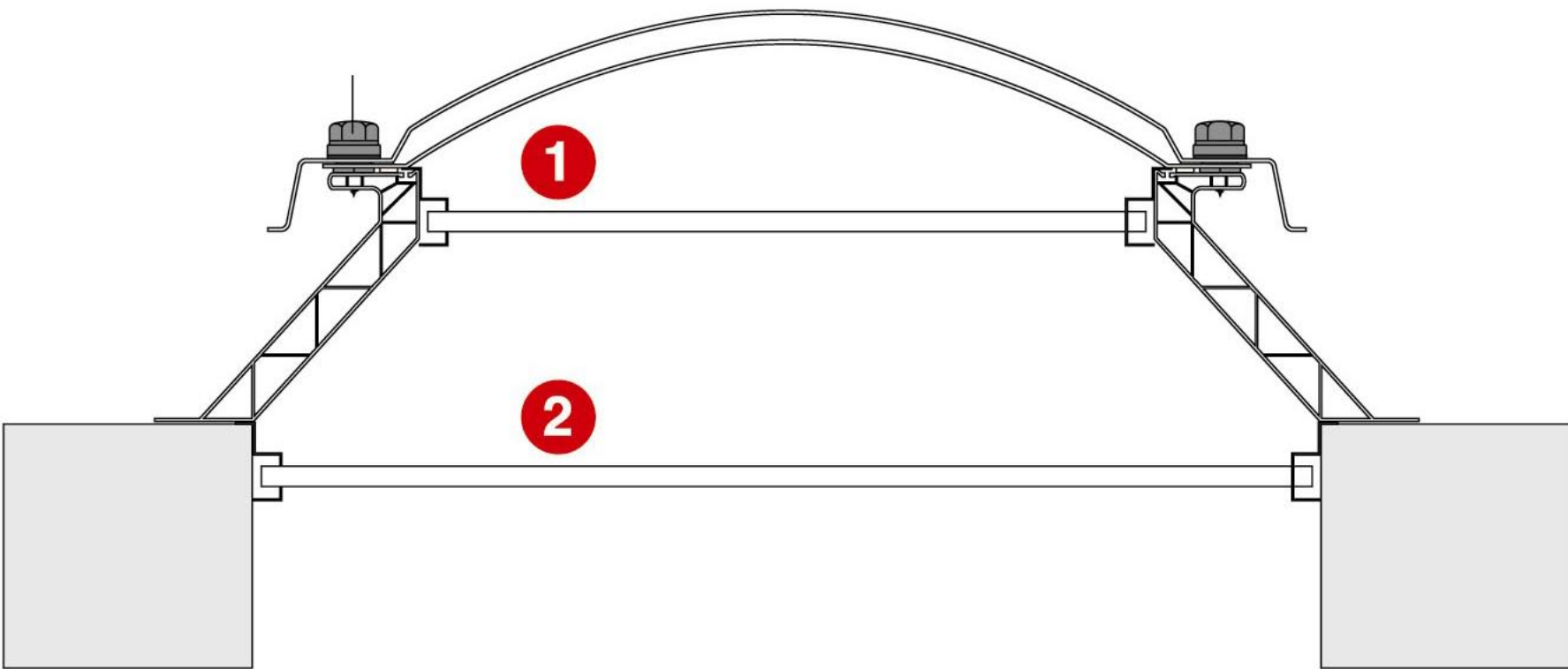
Detail SAVE2000 Anti- inbraak/doorvalbeveliging
