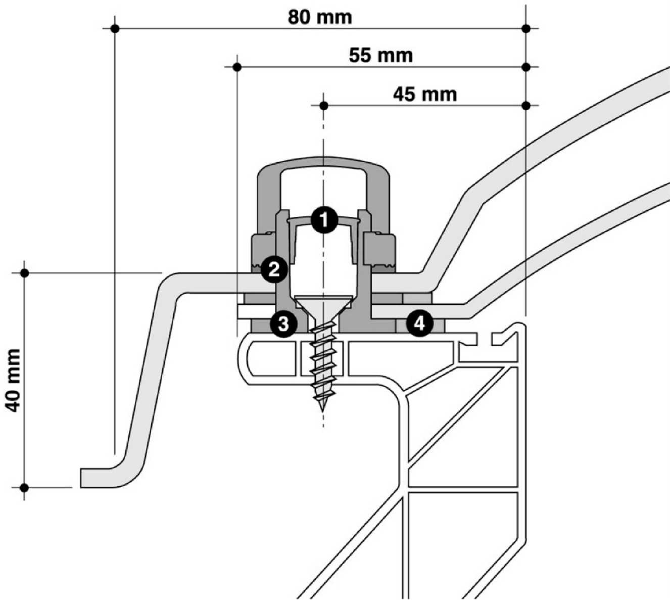
Detail SAVE2000 koepelbevestiging
